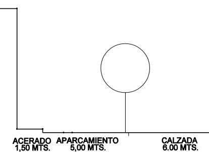
VIARIO V3. ANCHO TOTAL = 14,00 MTS.
