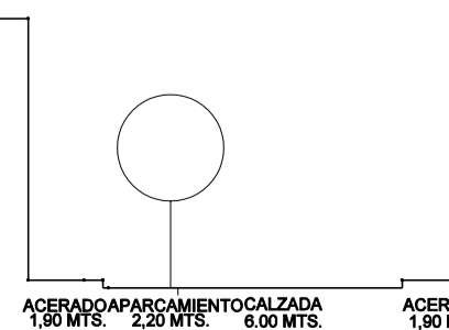
VIARIO V2. ANCHO TOTAL = 12,00 MTS.
